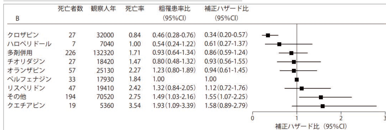
図4 Tiihonen J et al.: 11-year follow-up of mortality in patients with schizophrenia: a population-based cohort study (FIN11 study) : The Lancet 374, Issue 9690: 620-627, 2009 https://www.sciencedirect.com/science/article/pii/S014067360960742X?via%3Dihub
